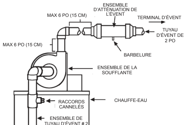
FIGURE 23 : Installation horizontale type
